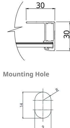
Frame Cross Section A-A
