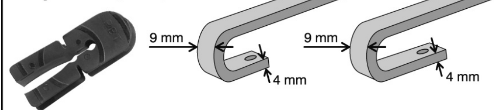
adaptor M9 (4 x 9)
