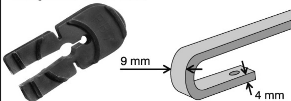
adaptor M4 (4 x 9)
