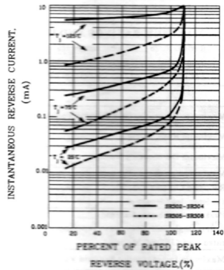
FIG.4-TYPICAL REVERSE CHARACTERISTICS
