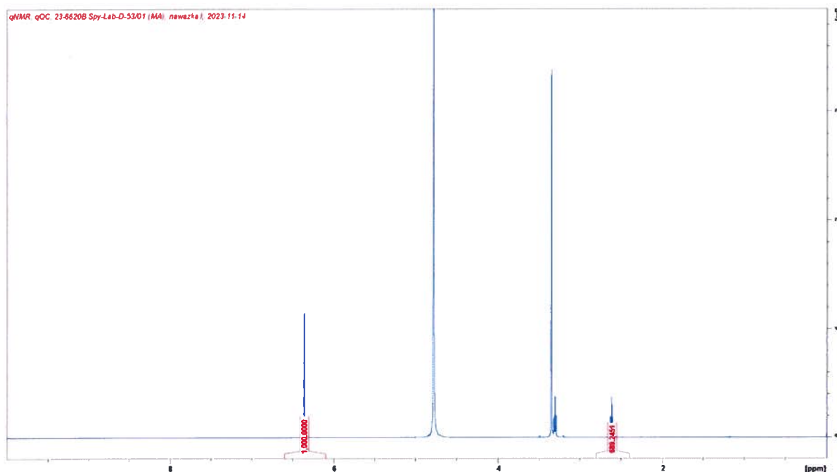
Widmo ^1\text{H} qNMR, meldonium dihydrate CAS: 86426-17-7 (23-6620B), kwas maleinowy (Spy-Lab-D-53/01) w \text{D}_2\text{O} .
