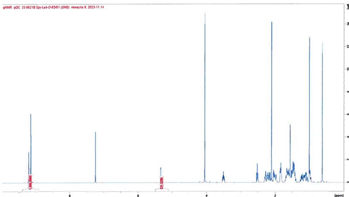
Widmo ^1\text{H} qNMR, pregnenolone CAS: 145-13-1 (23-6621B), 3,5-dinitrobenzoesan metylu (Spy-Lab-D-65/01) w \text{CDCl}_3 .
