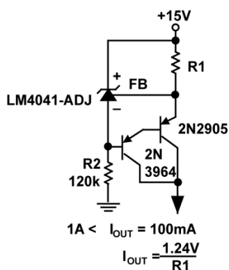
Figure 8. Current Source
