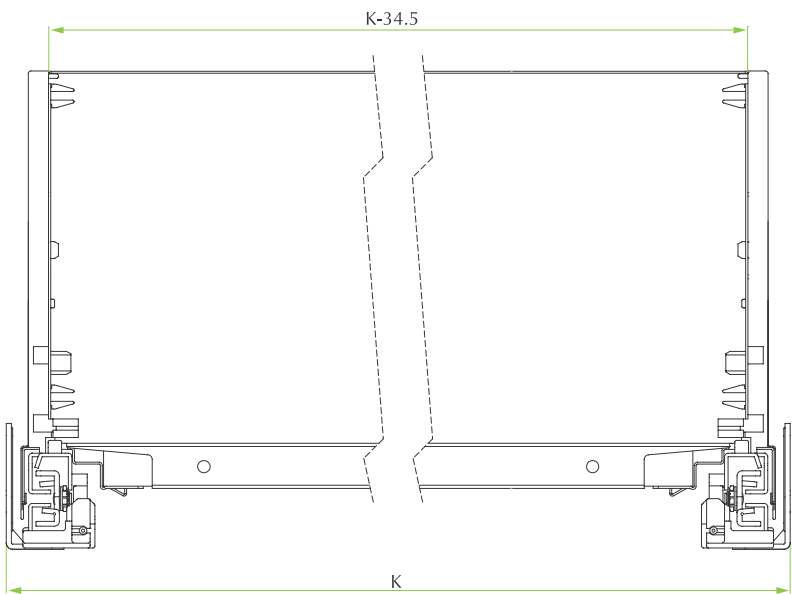
Drawer H180
