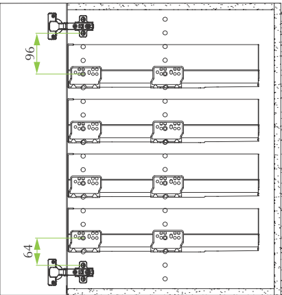
Drawer H90
