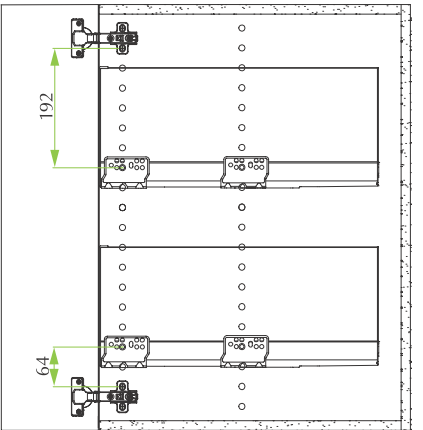
Drawer H180
