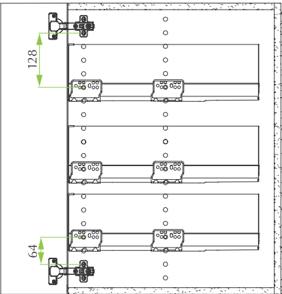
Drawer H120
