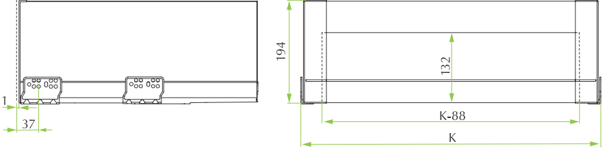
Drawer H180
