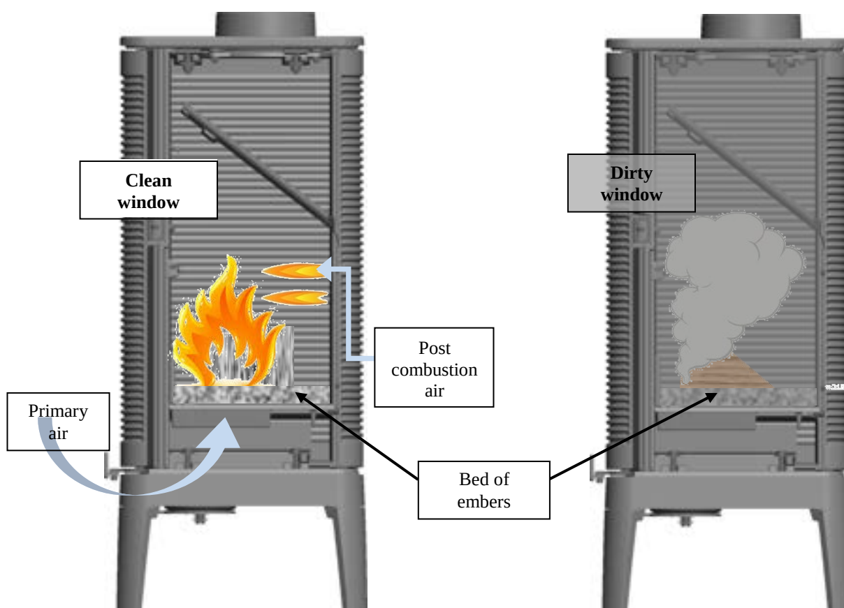
Principle diagram
