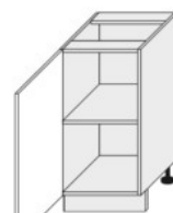
D1D 40 (400/820/500)
