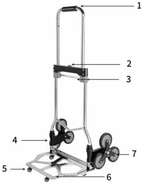
1.Handle 2.Push Button 3.Connector 4.Rotating Shaft 5.Universal Wheel 6.Tray 7.Climbing Wheel
