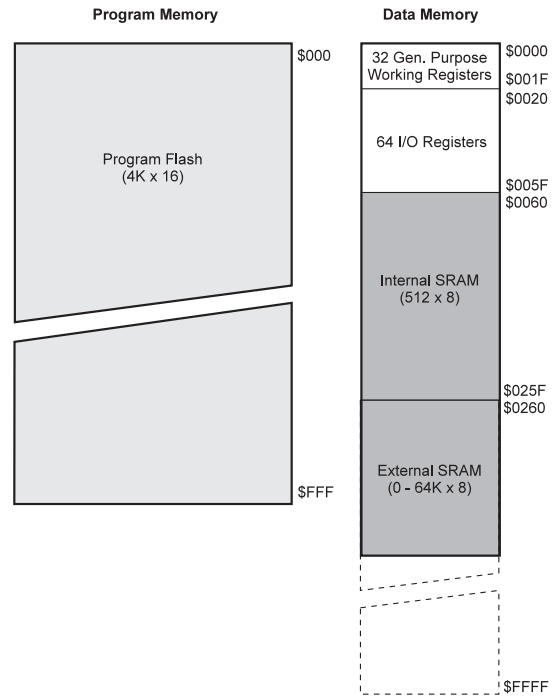
Figure 5. Memory Maps
