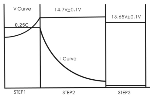
Charge Curves
