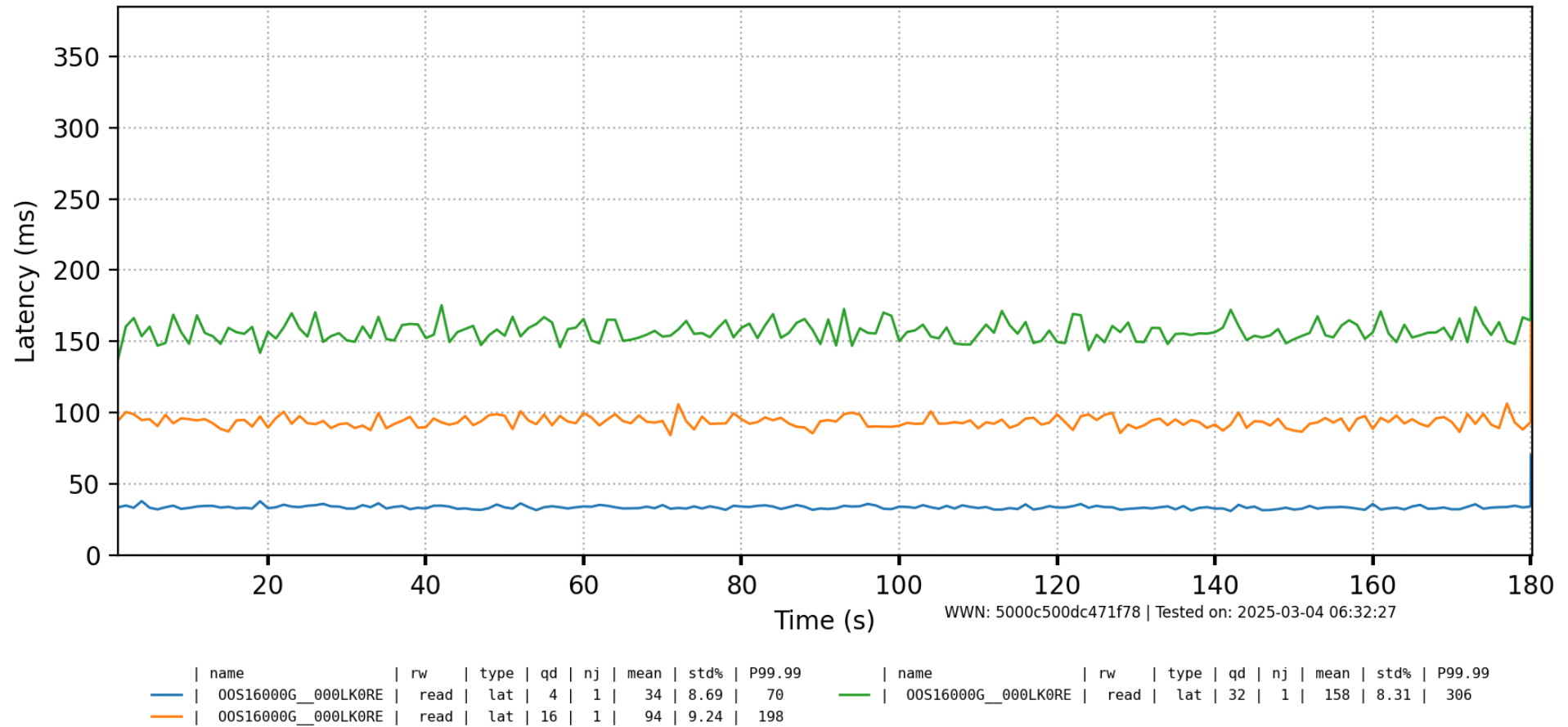
Figure 8. randread-g-lat-d
