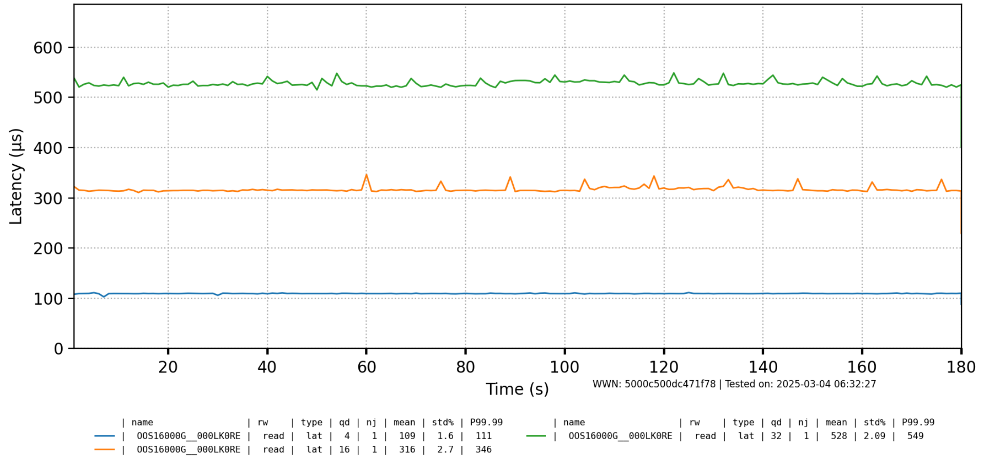
Figure 3. read-g-lat-d
