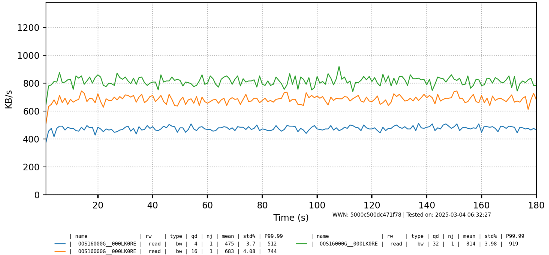
Figure 6. randread-g-bw-d
