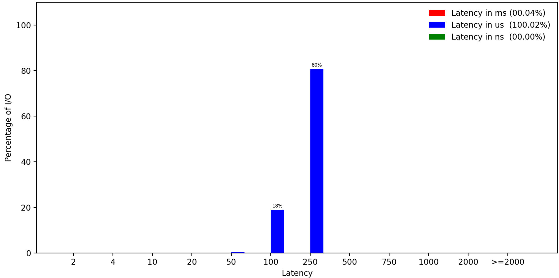
Figure 5. read-H
