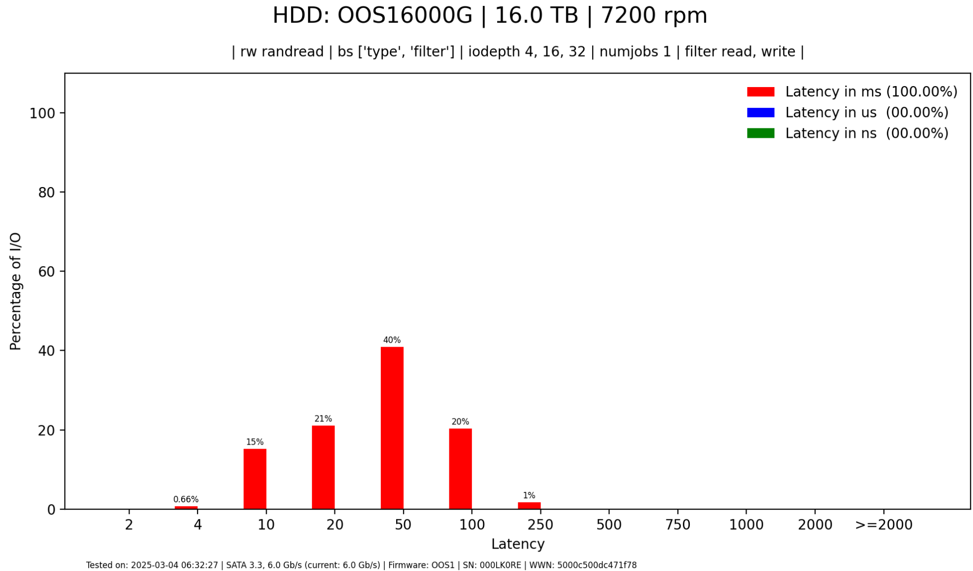
Figure 10. randread-H
