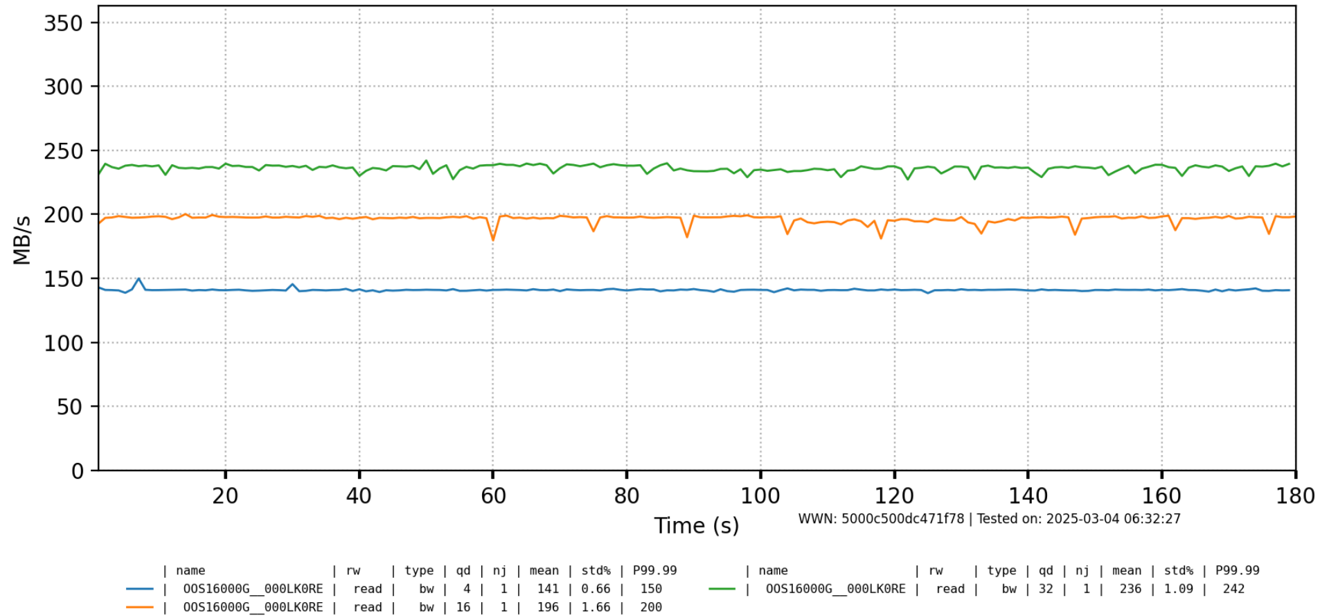
Figure 1. read-g-bw-d
