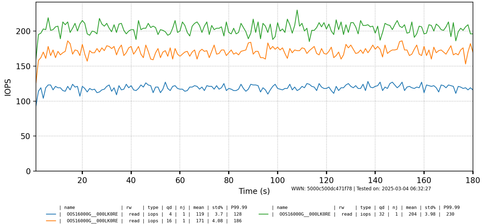
Figure 7. randread-g-iops-d
