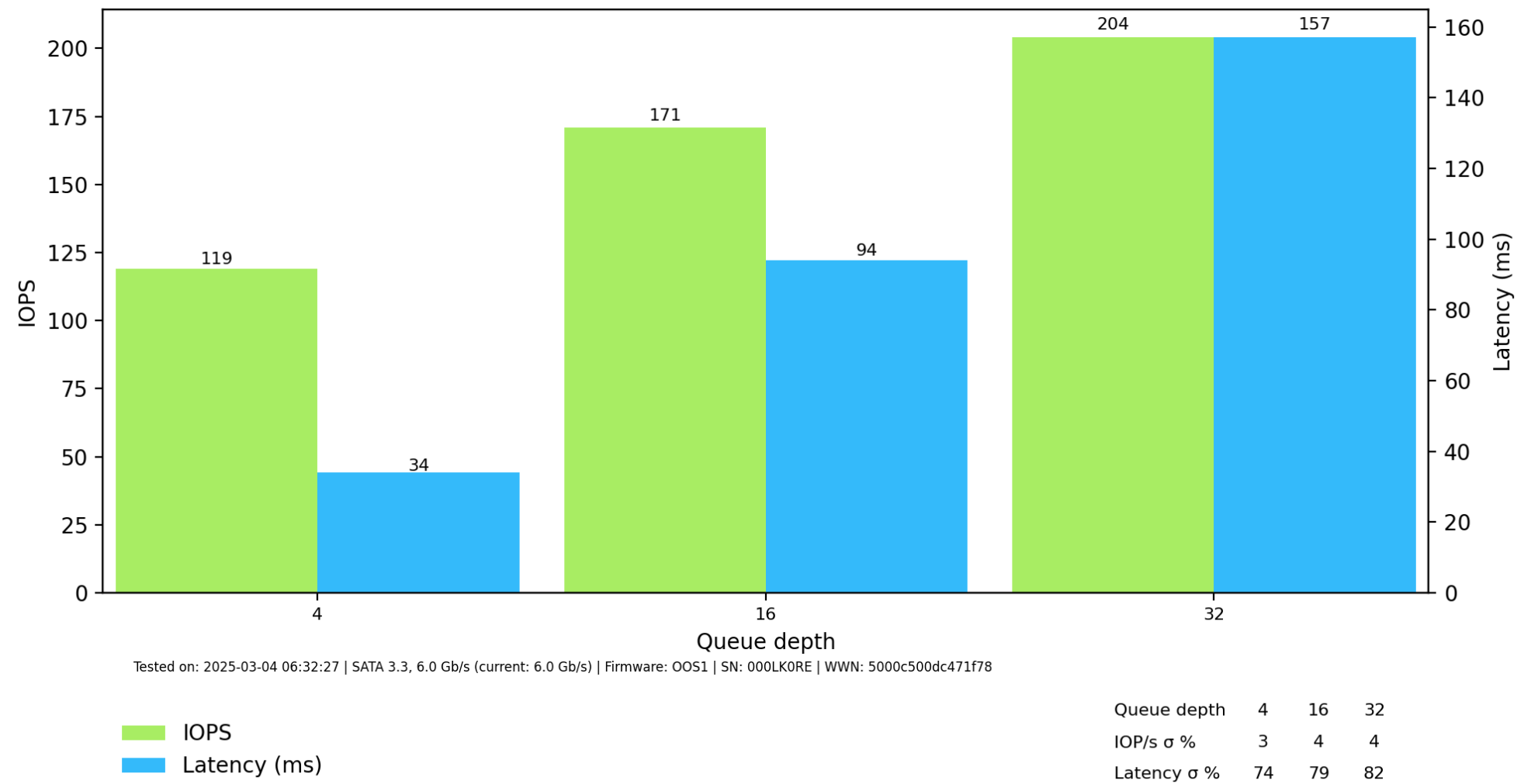
Figure 9. randread-l
