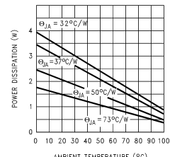
Maximum Power Dissipation (TO-263) (Note 3)
