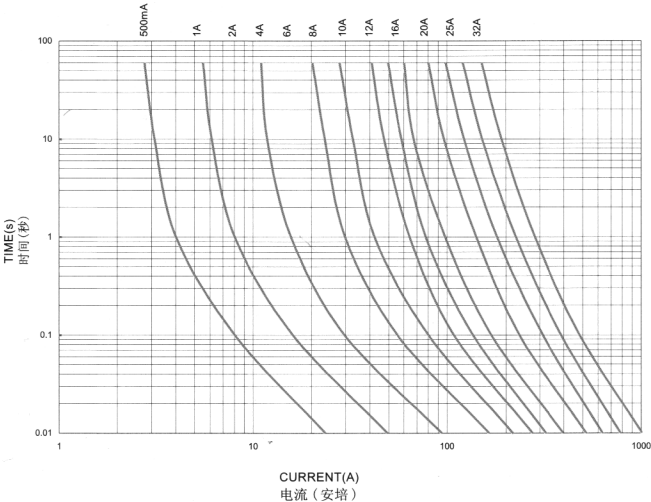
HC10aM平均 I-T 曲线图 (仅供参考) HC10aM AVERAGE I-T CHARACTERISTICS CURVE (FOR REFERENCE)
