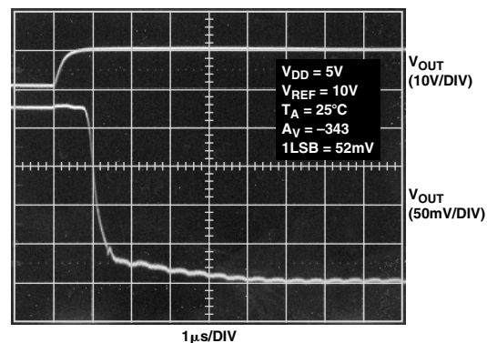
TPC 14. AD5544 Small Signal Settling Time
