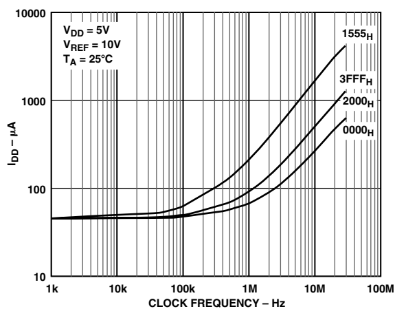
TPC 16. AD5554 Power Supply Current vs. Clock Frequency
