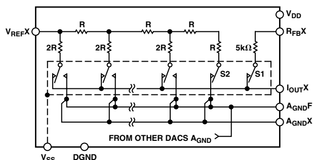
Figure 4. Typical Equivalent DAC Channel
