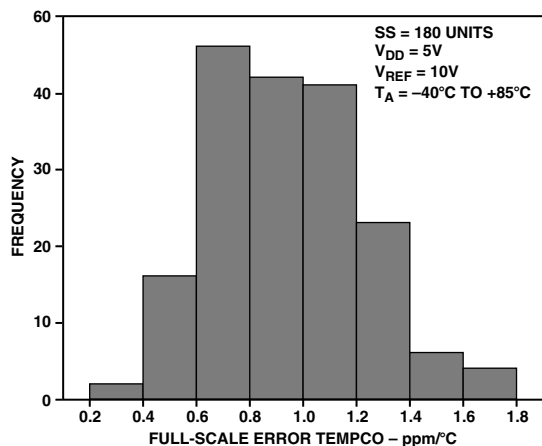
TPC 11. AD5544 Full-Scale Tempco (ppm/ ^{\circ}C )
