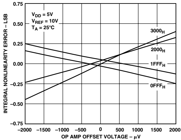
TPC 5. AD5554 Integral Nonlinearity Error vs. Op Amp Offset
