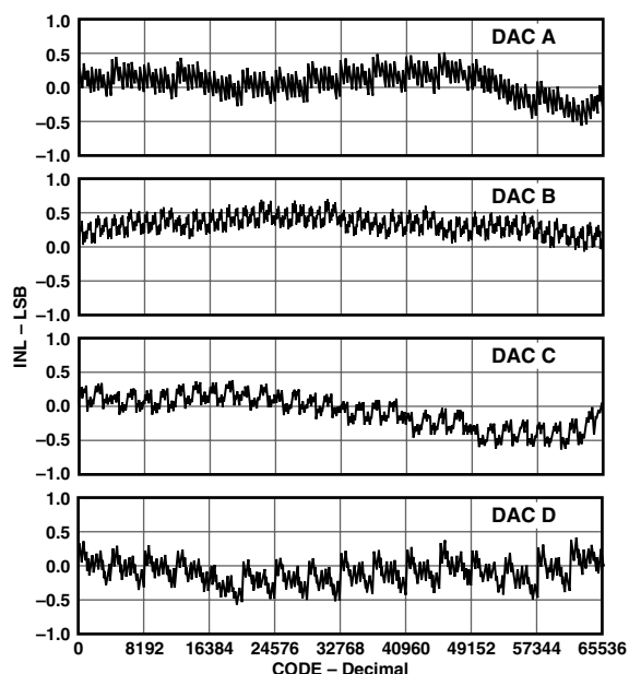
Figure 1. AD5544 INL vs. Code Plot ( T_A = 25^\circ\text{C} )
