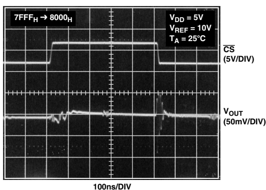
TPC 12. AD5544 Midscale Transition
