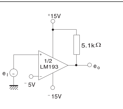
Figure 18. Comparator with a negative reference
