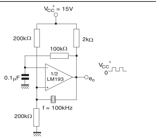
Figure 16. Crystal controlled oscillator
