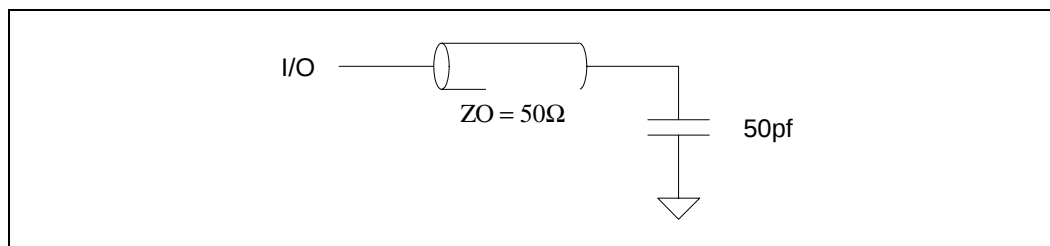
Figure 22: AC Test Load
