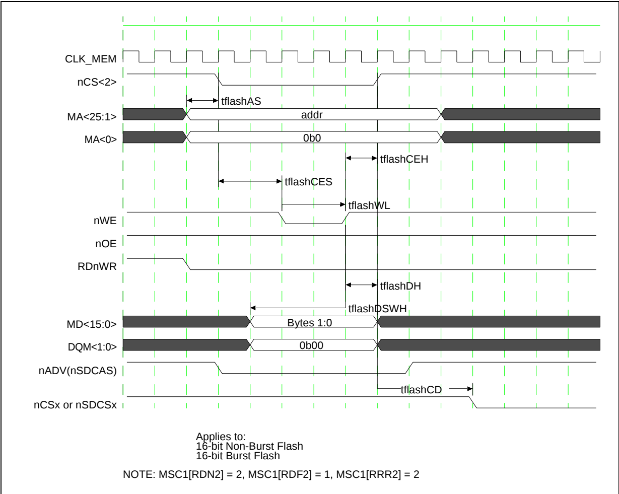
Figure 42: 16-Bit Flash Write Timing
