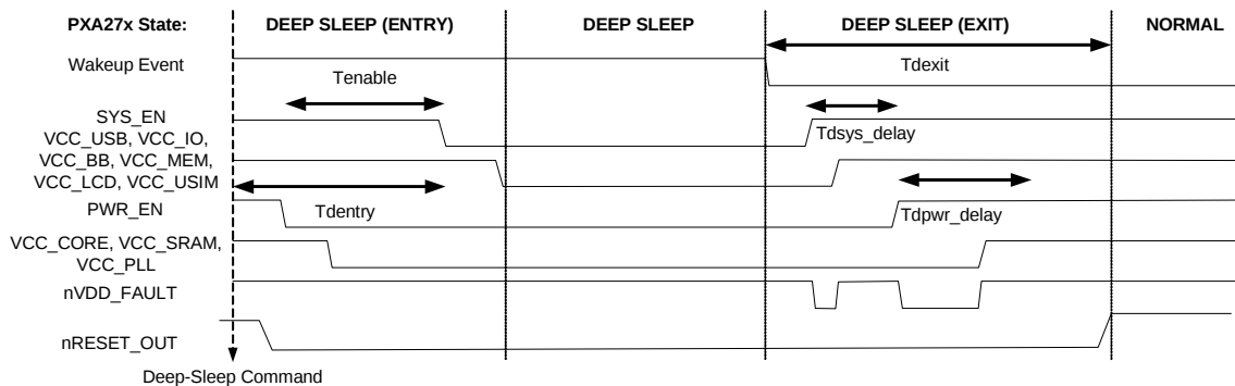
Figure 27: Deep-Sleep-Mode Timing
