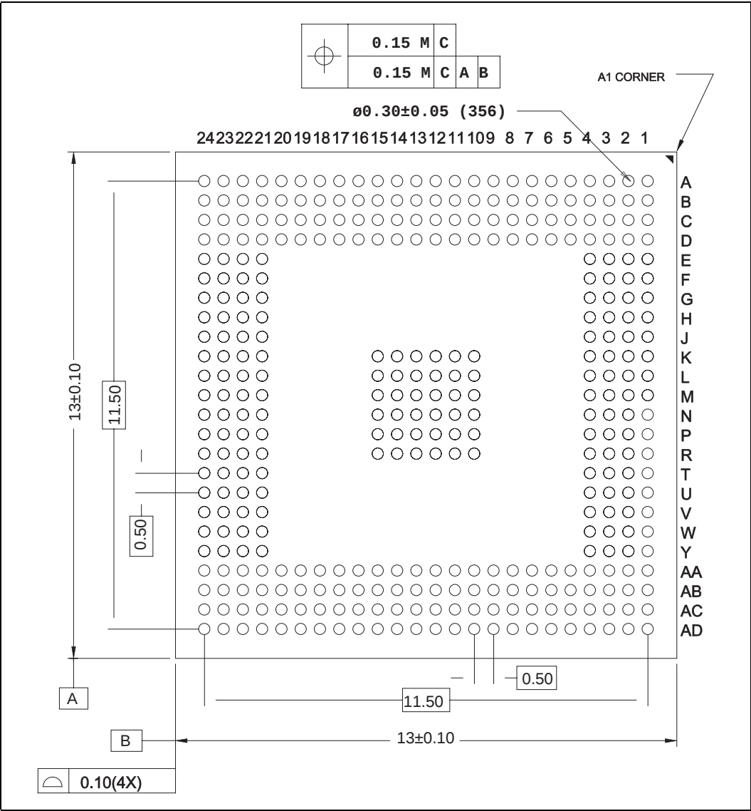
Figure 4: 13x13mm VF-BGA Marvell® PXA270 Processor Package, bottom view
