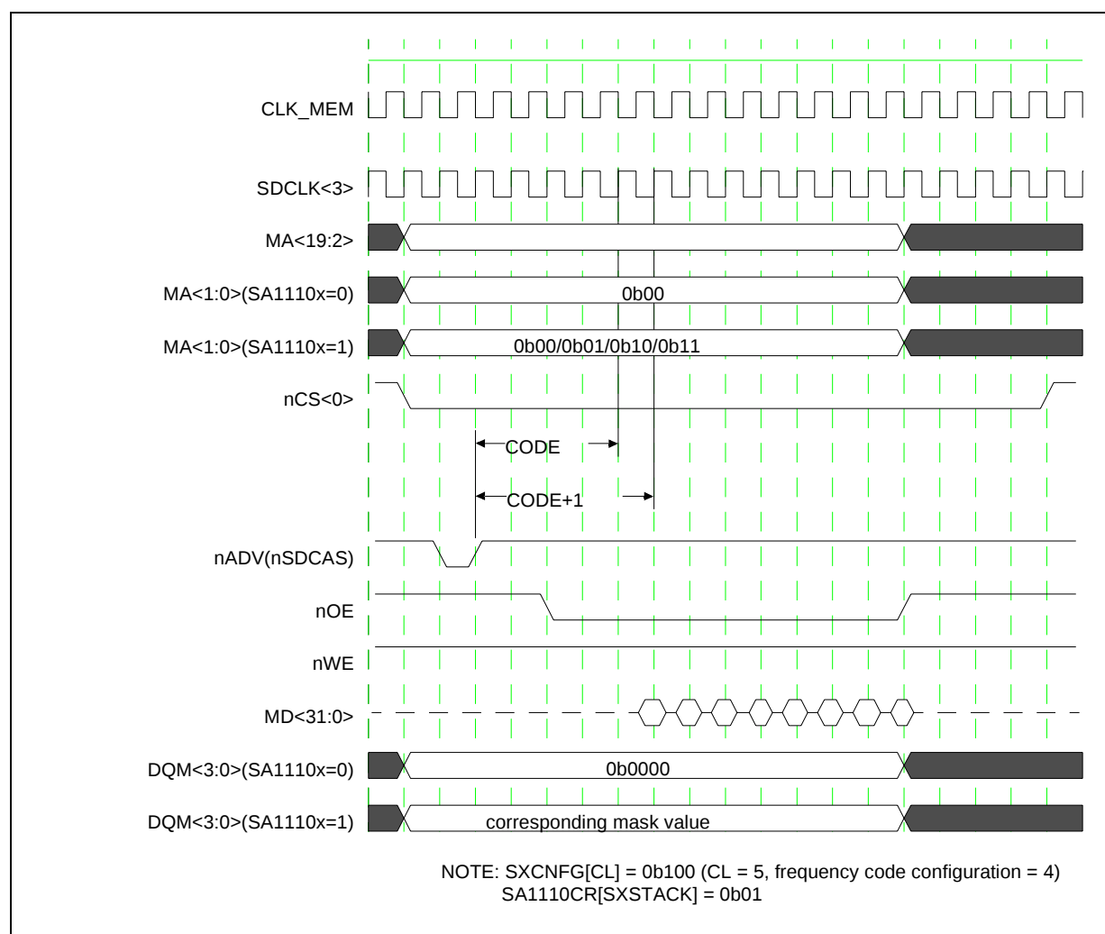
Figure 37: Synchronous Flash Stacked Burst-of-Eight Read Timing
