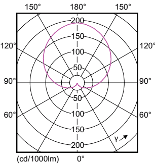
CorePro LEDbulb ND 5-40W A60 E27
