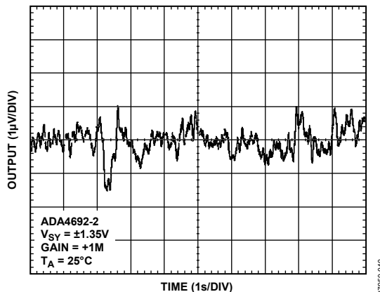
Figure 40. 0.1 Hz to 10 Hz Noise
