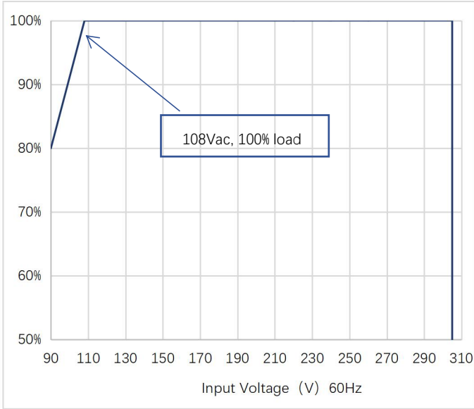
Load Derating Curve
