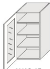
W4S 45 (450/960/325)
