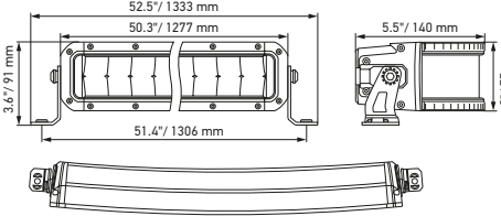
Black Magic 50" Double Row Curved Lightbar
