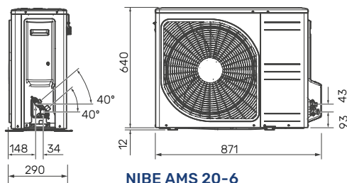
NIBE AMS 20-6
