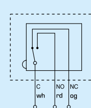
Option, Auxiliary switch The actuators are fitted with two separate cables, one cable for actuator regulation and one for the auxiliary switch.
