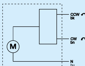
Actuator 3-point, with fixed cable
