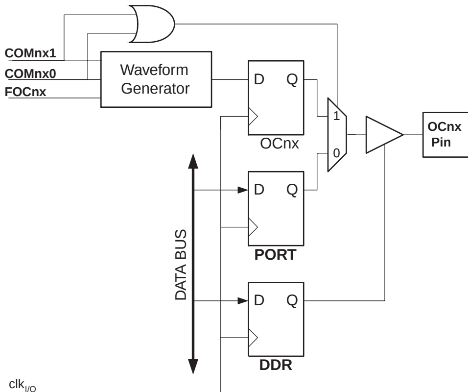
Figure 51. Compare Match Output Unit, Schematic
