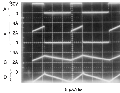
Switching Waveforms
