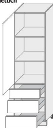
D/14/DP/3A (600/2070/565)
