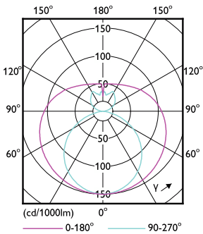
Light Distribution Diagram - CorePro LEDtube 1200mm 15.5W 840 T8 CL
