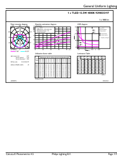
General uniform lighting - CorePro LEDtube 1200mm 15.5W 840 T8 CL
