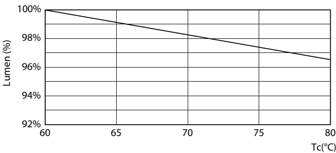
Lumen Maintenance Diagram - CorePro LEDtube 1200mm 15.5W 840 T8 CL
