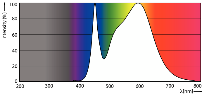
Spectral Power Distribution Colour - CorePro LEDtube 1200mm 15.5W 840 T8 CL
