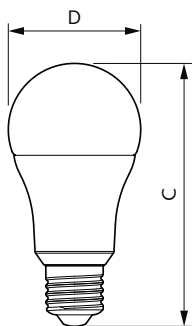
LEDbulb ND 13-100W A67 E27 827 2CT
