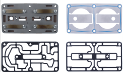
440.01.1300 Plate Kit
