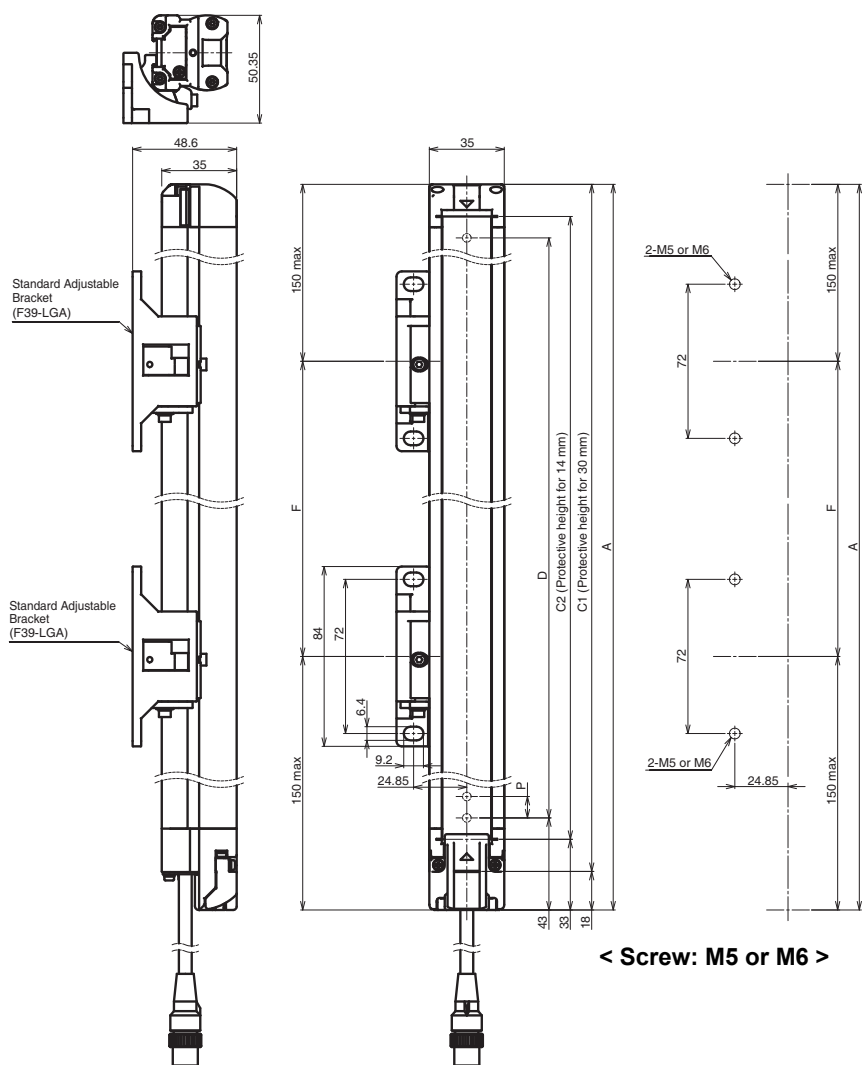
F3SG-□RA□□□□-30 Series
