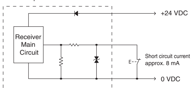
<NPN Output>
