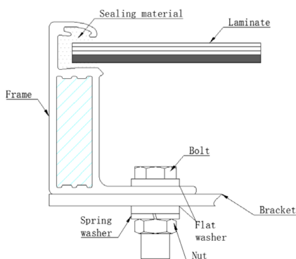
Fig. 8.1 Bolt installation diagram
