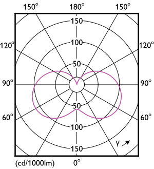
Light Distribution Diagram - CorePro candle ND 2.8-25W E14 840 B35 FR
