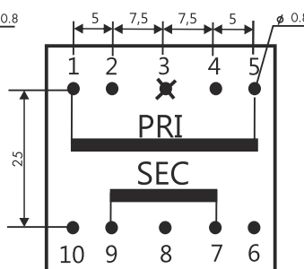
TEZ 6,0
