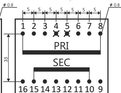
TEZ 40; 50
