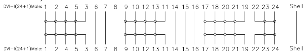
Soldered Drawing:
