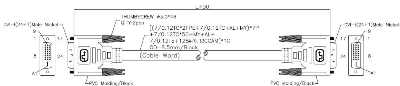
Soldered Drawing:
