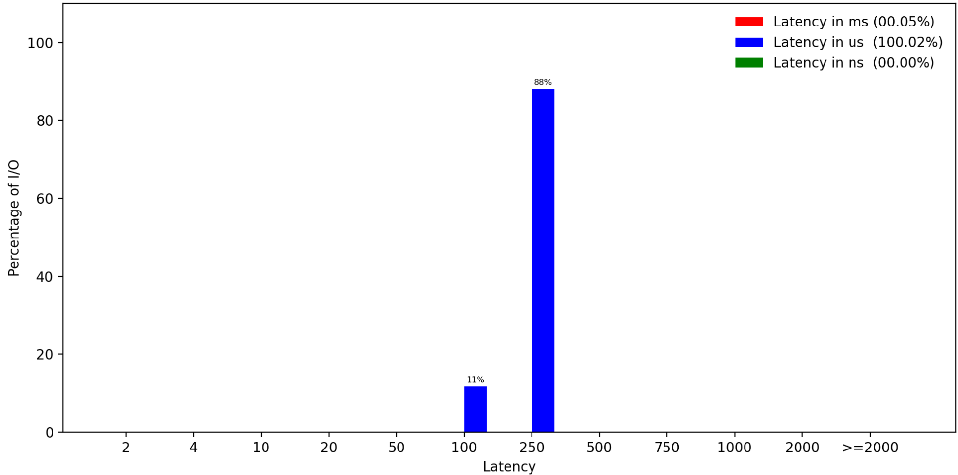
Figure 5. read-H
