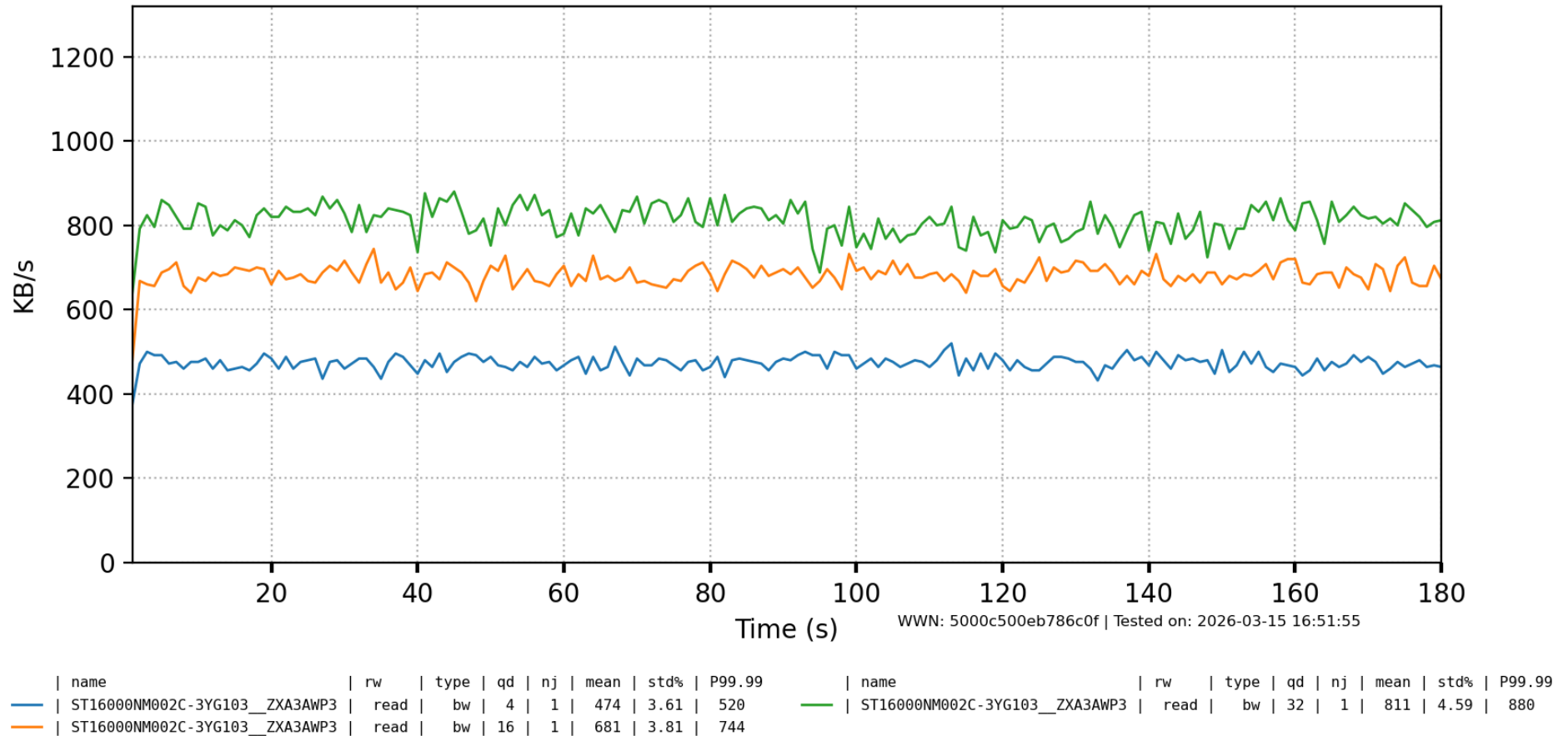
Figure 6. randread-g-bw-d
