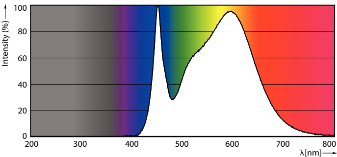
Spectral Power Distribution Colour - LEDbulb ND 4.9-40W A60 E27 840 2CT
