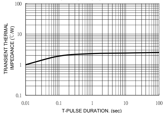
FIG. 6- TYPICAL TRANSIENT THERMAL CHARACTERISTIC
