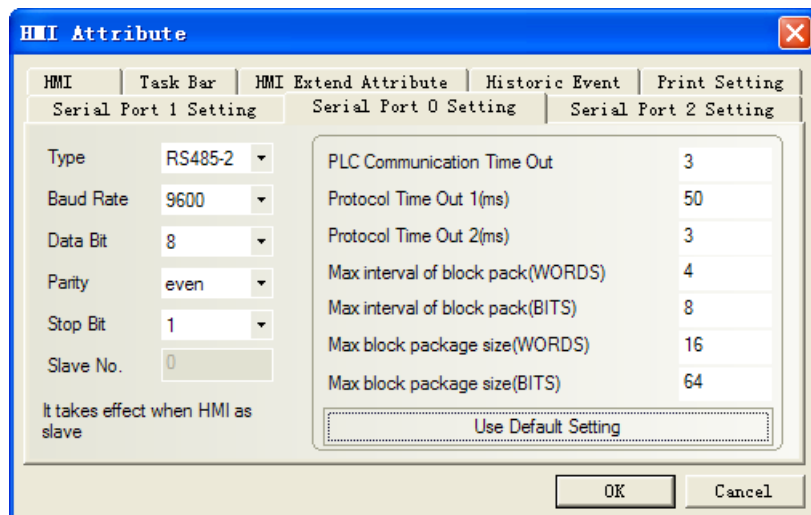
RS485 communication
