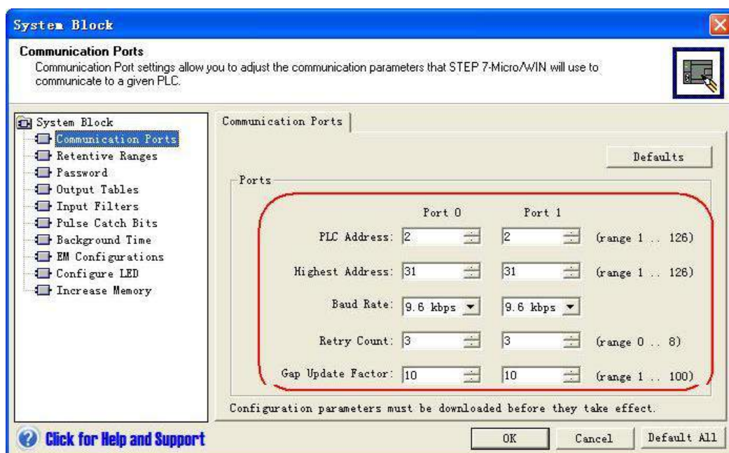
PLC Setting
