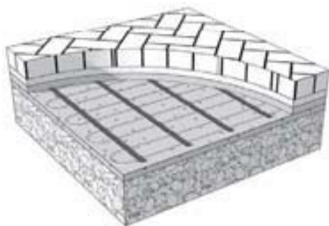
MA ICE-30 cable under paving stones
