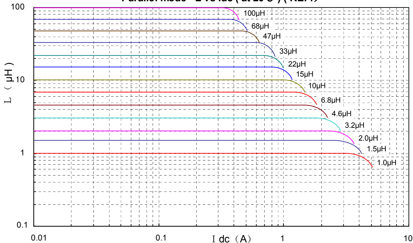
Parallel mode L vs I dc ( at 20℃ ) ( REF. )
