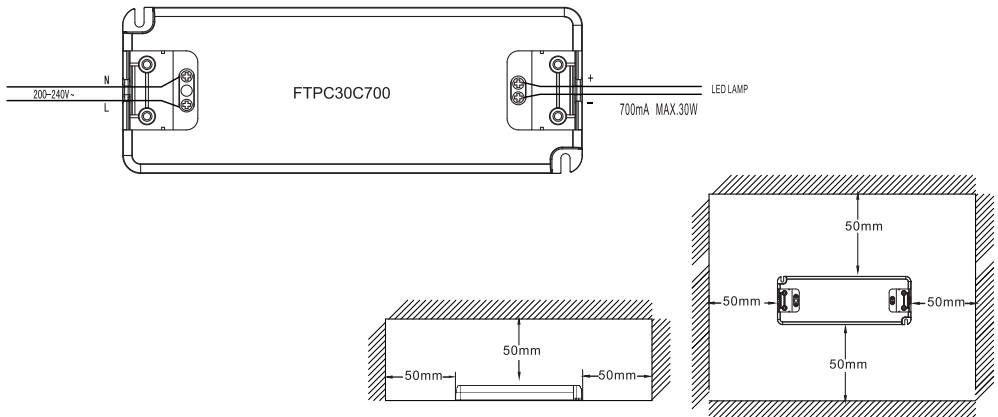
Mounting Location Dimension
