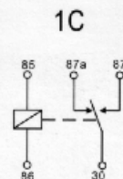
WIRING DIAGRAM (BOTTOM VIEW)
