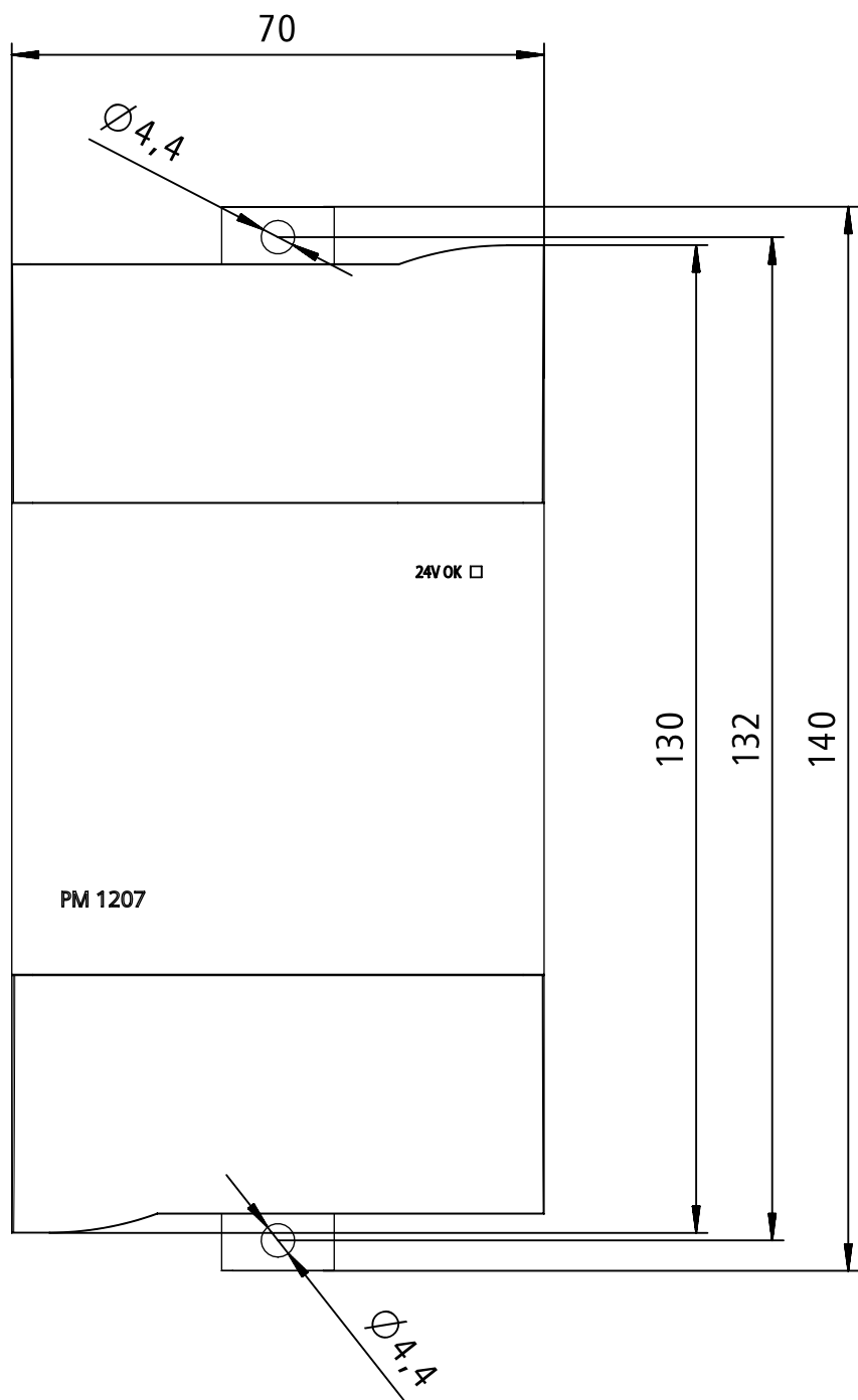
Montageoption/Mounting option
