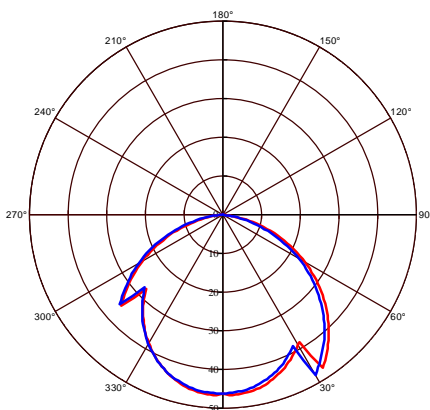
↳ C0 Plane beam angle(50%) 119.9(DEG) C90 Plane beam angle(50%):118.8(DEG)
