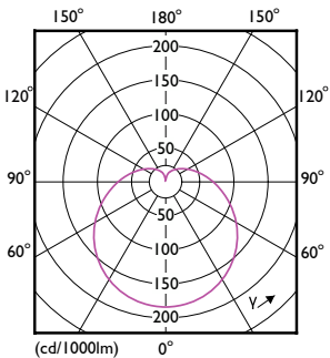
Light Distribution Diagram - LEDbulb ND 8-60W A60 E27 827 6CT
