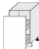
D1D 40 + cargo 40 (400/820/500)
