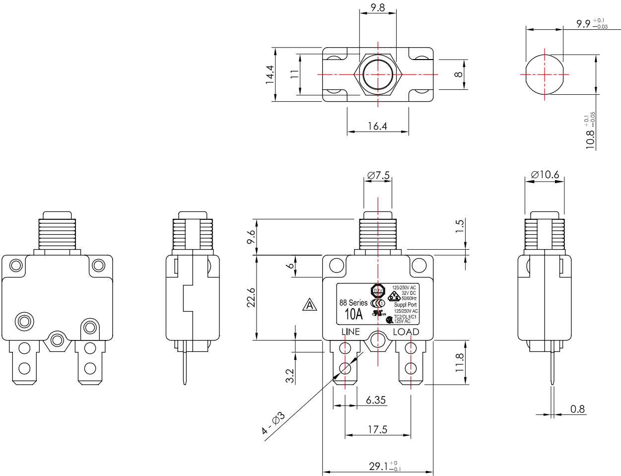
PANEL CUTOUT
