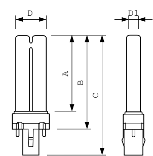
TUV PL-S 9W/2P
