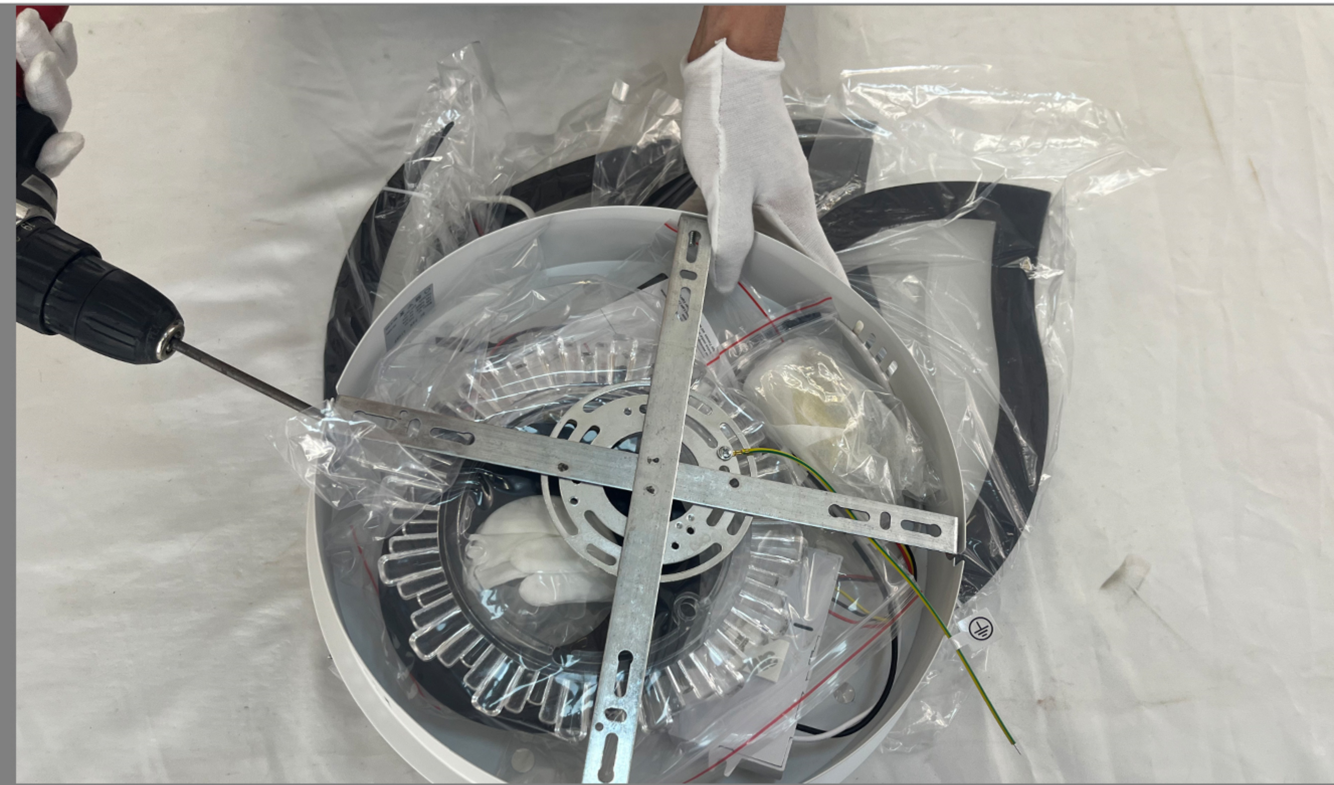
Step 1: Remove the mounting plate with screwdriver.
