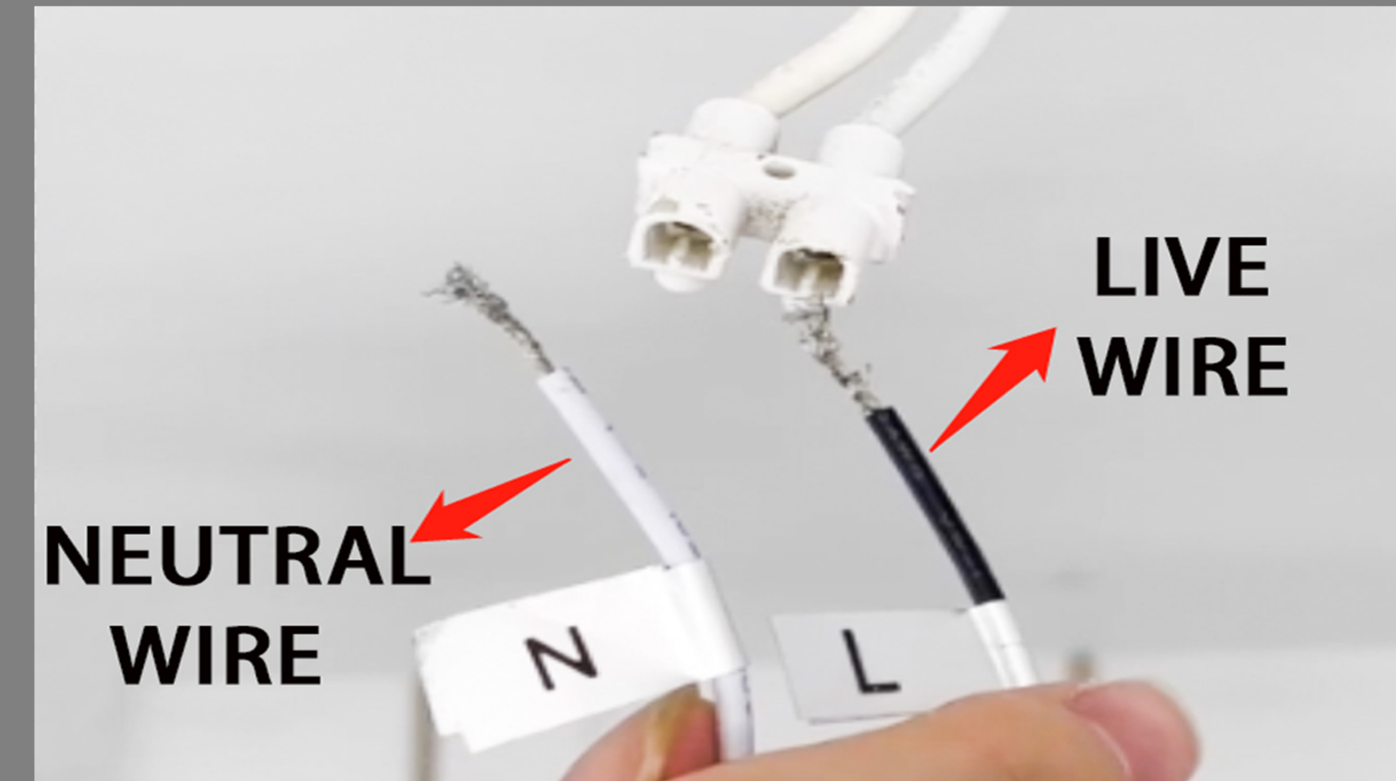
Step 8: Fix the light mounting plate to the ceiling. And connect converter AC Wires.
